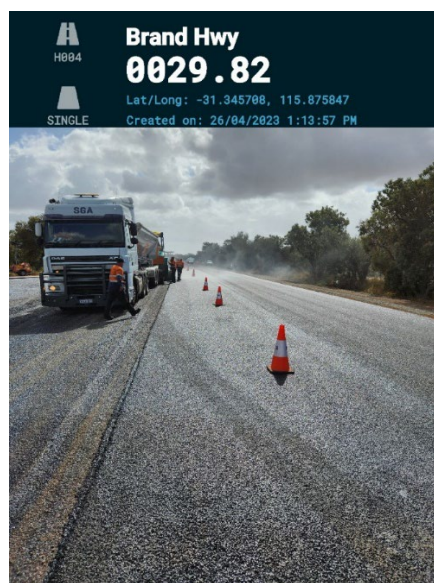
Asphalt Workers working within 1.2m of Live Traffic
